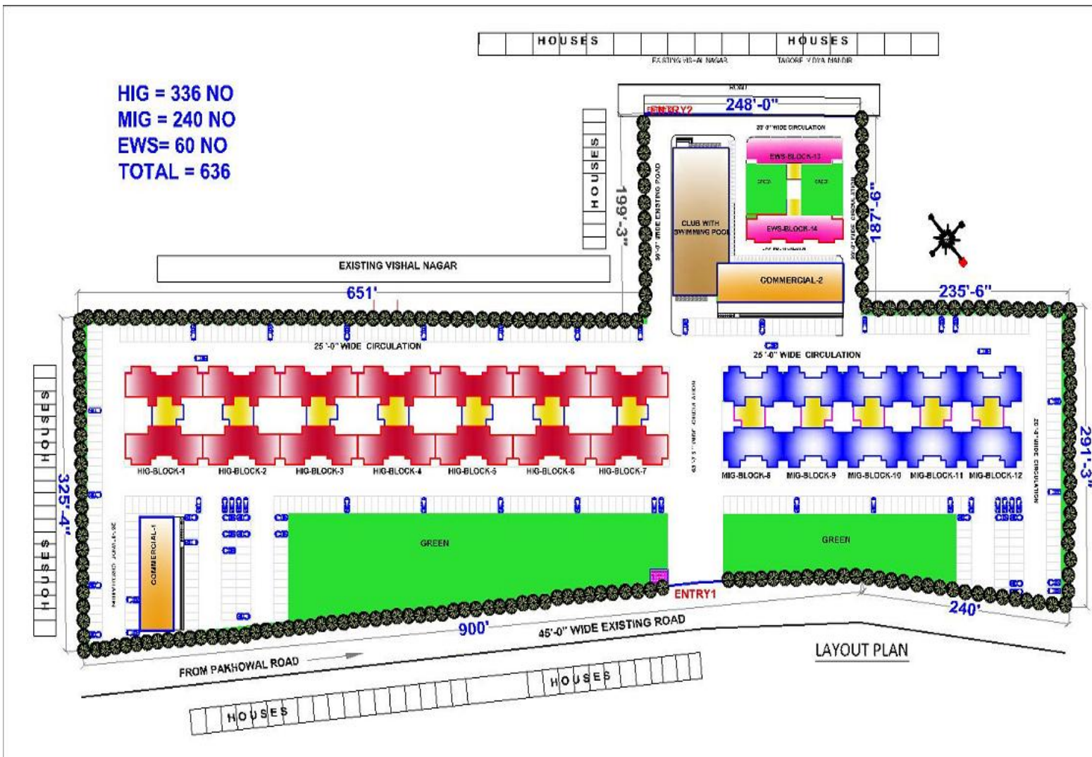
SITE PLAN
